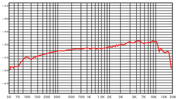
Spectrum Graph
