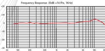
Spectrum Graph
