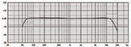
Frequency Response
