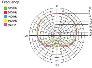
Polar Pattern
