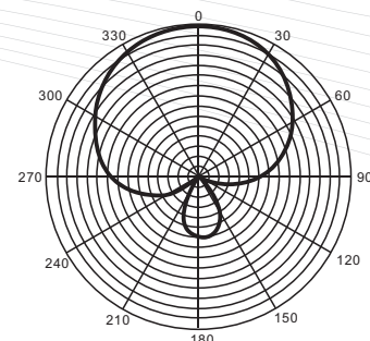
Polar Pattern
