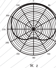
Polar Patterns
